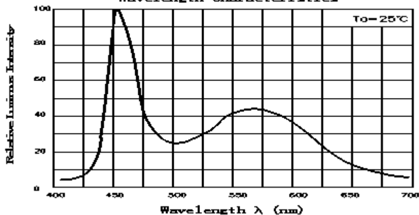
Wavelength Characteristics
