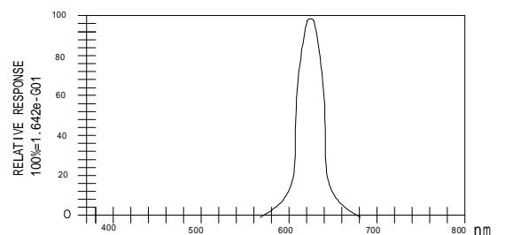
Luminous Spectrum (Ta=25°C) SPECTRAL RADIANCE
