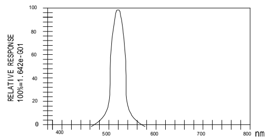
Luminous Sperttrum(Ta=25°C) SPECTRAL RADIANCE
