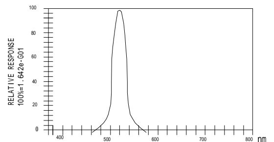
Luminous Spectrum (Ta=25°C) SPECTRAL RADIANCE
