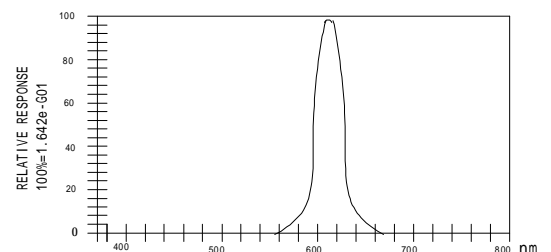
Luminous Spertum ( T_a=25^{\circ}\text{C} ) SPECTRAL RADIANCE
