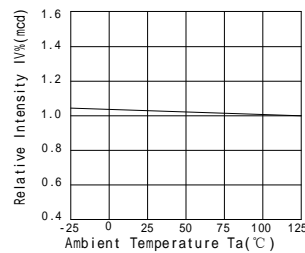
Relative Intensity vs. Ambient Temperature
