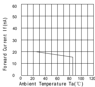
Forward Current vs. Ambient Temperature
