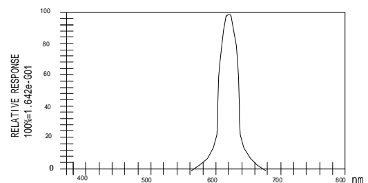
Luminous Spectrum ( T_a=25^{\circ}\text{C} )
