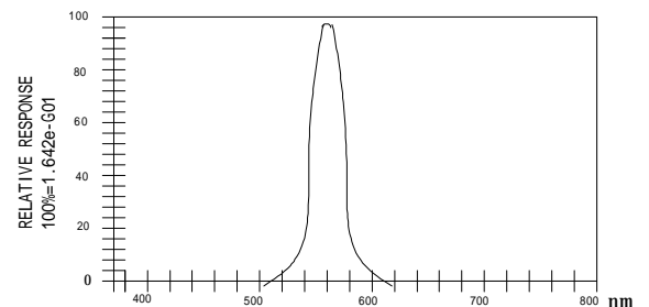
Luminous Sperrum ( T_a=25^{\circ}\text{C} ) SPECTRAL RADIANCE
