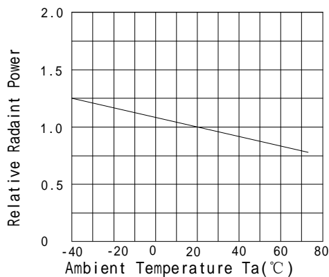
Radint Power Vs. Ambient Temperature
