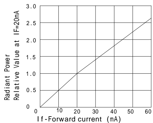
Radint Power Vs Forward Current
