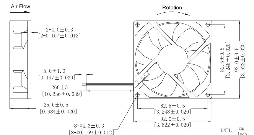
DIMENSIONS DRAWING
