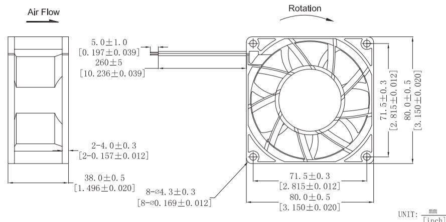
DIMENSIONS DRAWING
