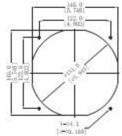
INLET SIDE
