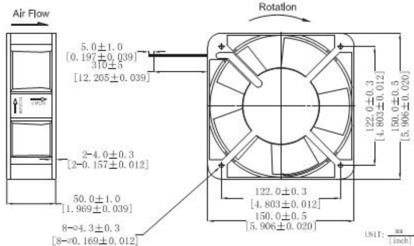
DIMENSIONS DRAWING
