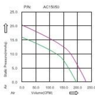
P&Q CURVE (AT RATED VOLTAGE)
