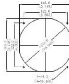
OUTLET SIDE
