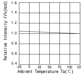
Relative Intensity vs. Ambient Temperature
