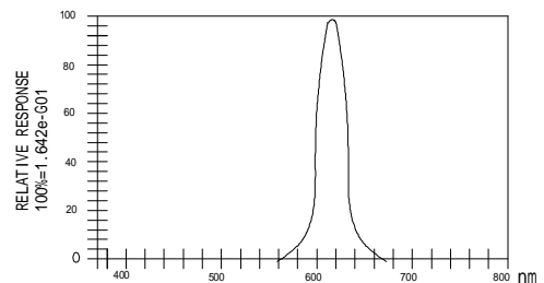
Luminous Spetrum ( T_a=25^{\circ}\text{C} ) SPECTRAL RADIANCE
