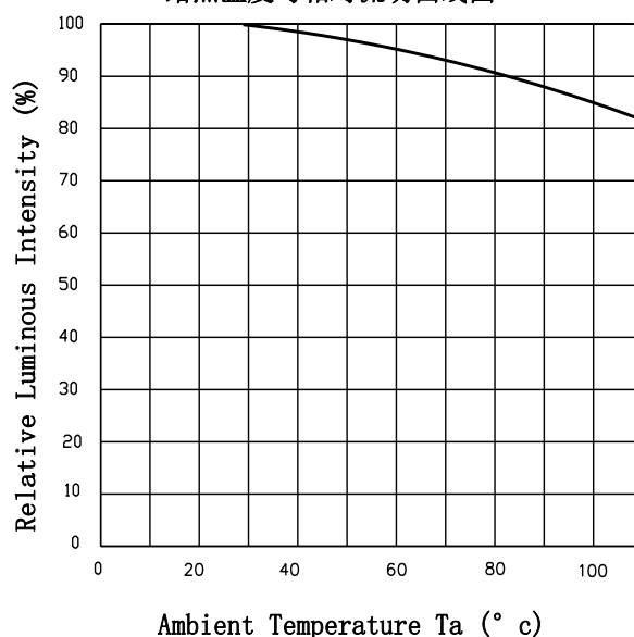
Relative Luminous Intensity - T_a
