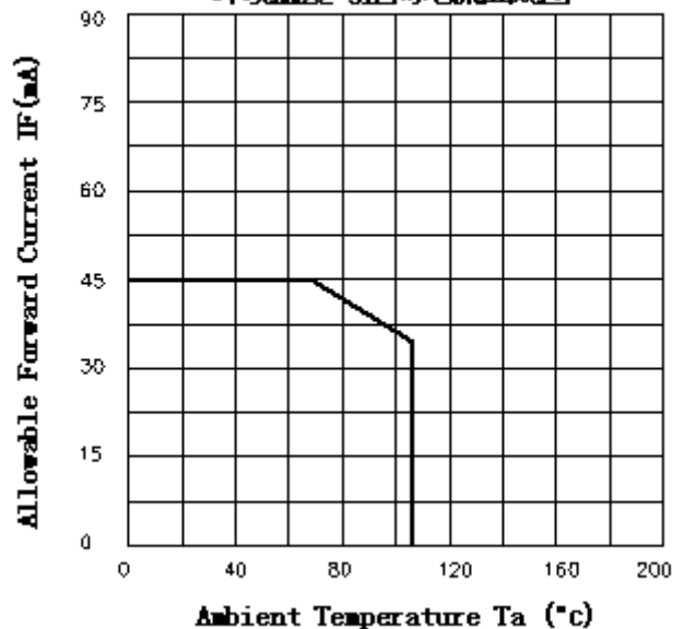
Allowable Forward Current - T_a
