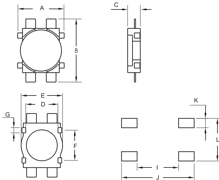
LAND PATTERNS
