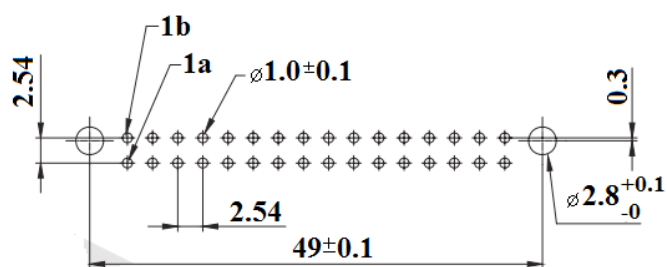
PCB Layout
