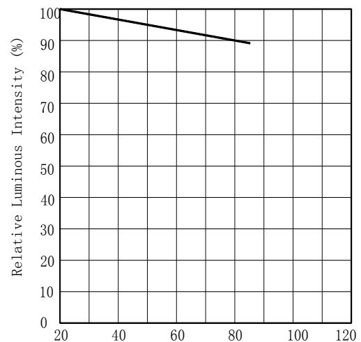
Relative Luminous Intensity - T_a
