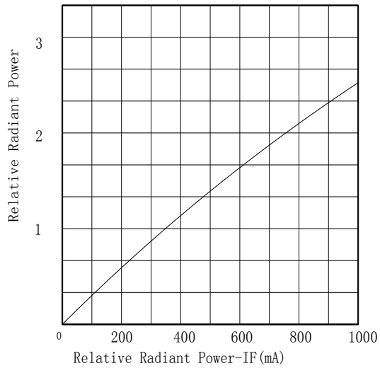
Relative Radiant Power-IF
