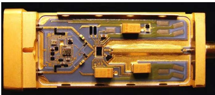
The InfiniiMax III and III+ probing system uses the same InP technology that enables high-bandwidth and low-noise oscilloscope measurements.
