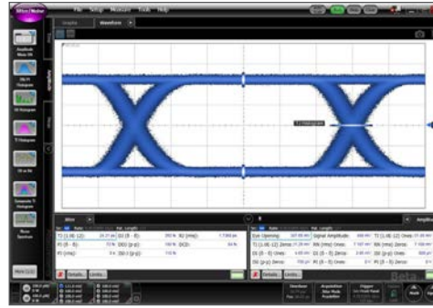
Precision jitter, amplitude, and frequency analysis capability
