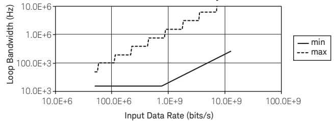
Selectable Loop Bandwidth vs Rate for 0.25 \leq \text{Transition Density} \leq 1
