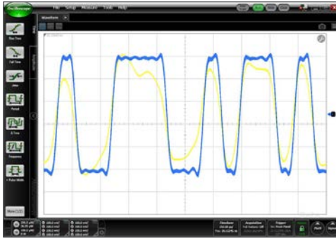
High-fidelity waveform characterization (Yellow: raw trace, Blue: de-embedded waveform)
