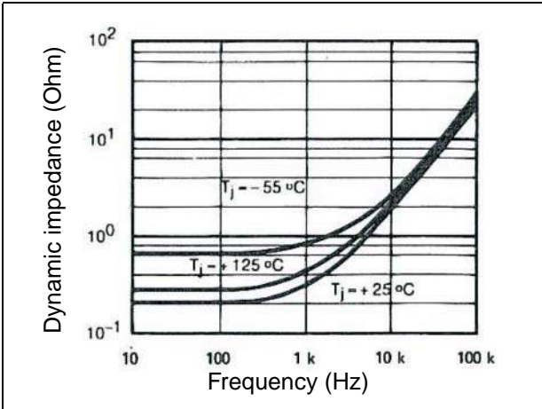
Figure 6. Dynamic impedance
