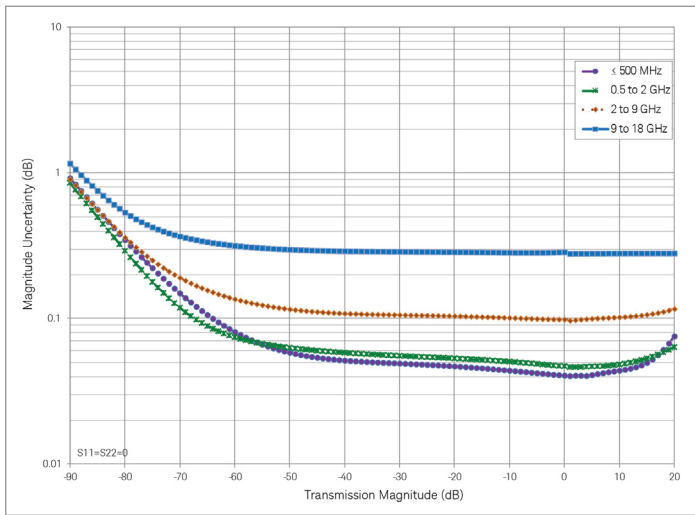
Transmission uncertainty (S21, S12)
