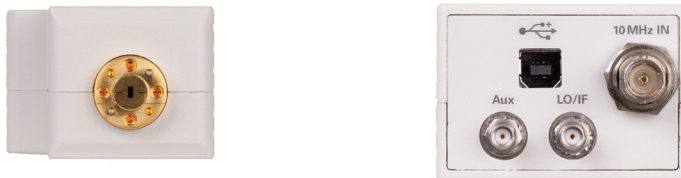
Figure 1. View of the M1971E/V/W connectors
