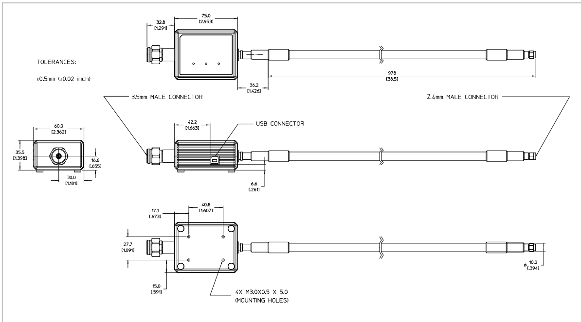
Figure 30. Mechanical dimensions for U7227F USB preamplifier
