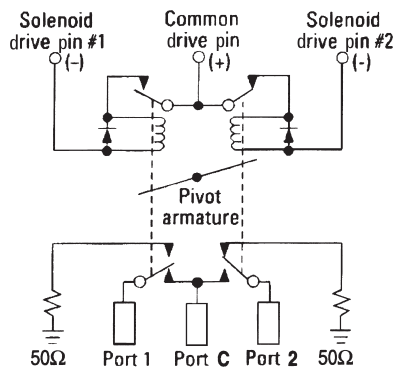
Figure 1. Keysight 8762
