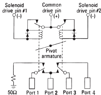
Figure 2. Keysight 8763
