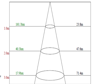
Illuminance at a distance (lux)
