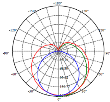
Light Distribution Curve:(cd)
