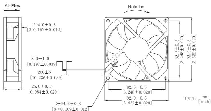
DIMENSIONS DRAWING
