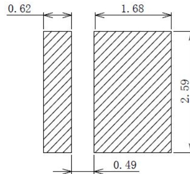
Recommended Soldering pad Layout (Unit: mm)
