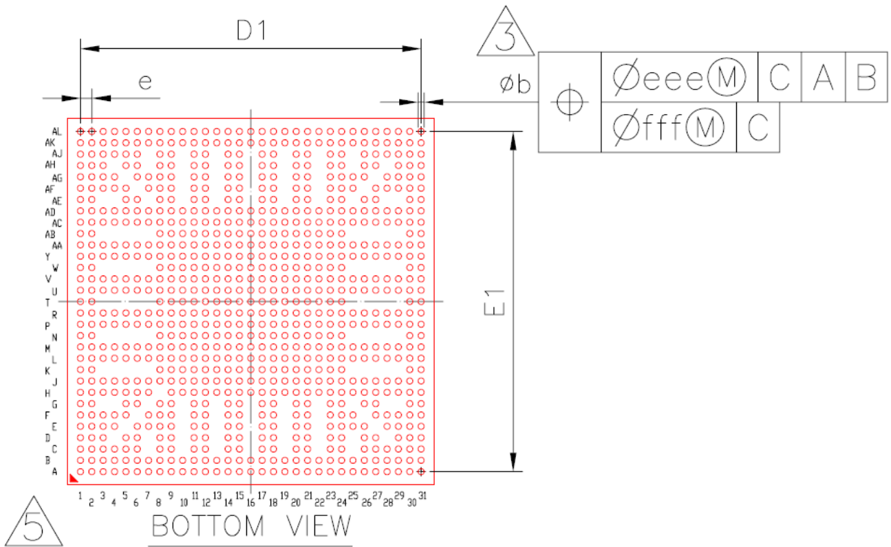
Fig. 2-2RK3399FCBGA828 Package Bottom View
