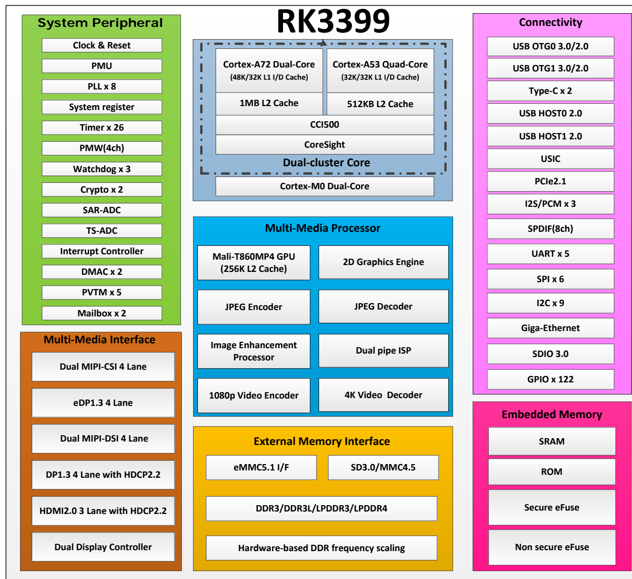
Fig. 1-1RK3399 Block Diagram
