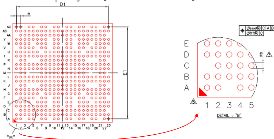
Fig. 4 RK3066 TFBGA453 Package Bottom View
