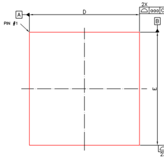
Fig. 2 RK3066 TFBGA453 Package Top View
