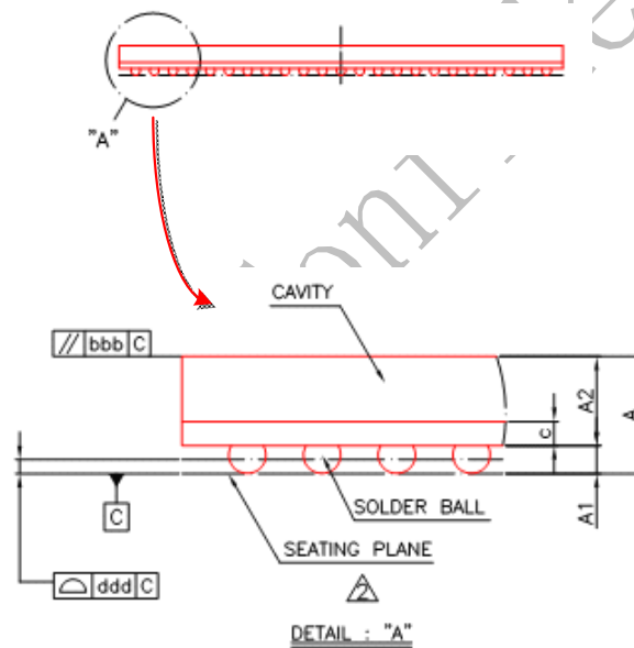
Fig. 2 RK3066 TFBGA453 Package Side View
