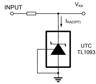
For I_{KA(OFF)}
