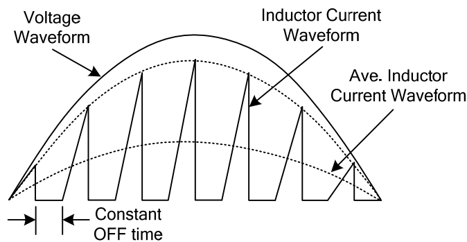
Figure 1. Power Factor Correction
