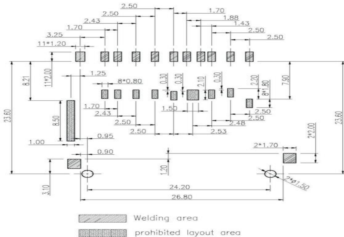
Recommend PCB Layout Drawing: (Unit:mm .X ± 0.15 .XX ±0.05 .XXX ± 0.02)
